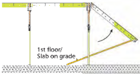
Step 1 Erect TABLA SHORING SYSTEM from floor slab.
