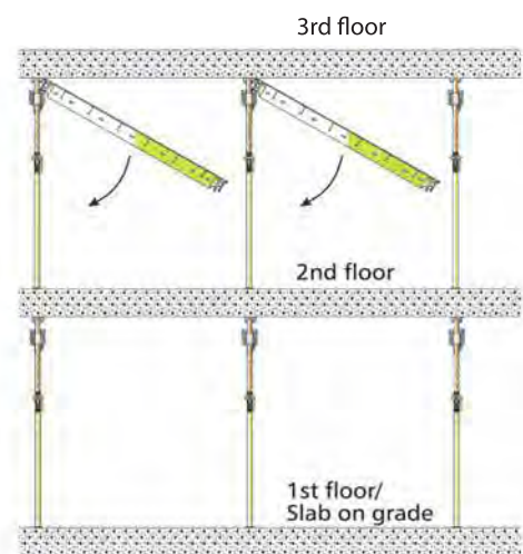
Step 6 Once concrete reaches 2000 psi, remove TABLA Panels from third floor. Leave TABLA Props undisturbed.
