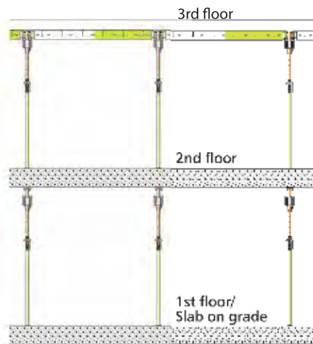
Step 5 Shoring for third floor complete, pour third floor.
