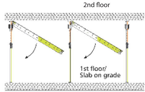
Step 3 Once concrete reaches 2000 psi, remove TABLA Panels. Leave TABLA Props undisturbed.
