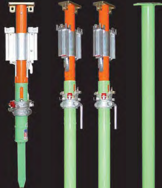
PH Pioneer Head
