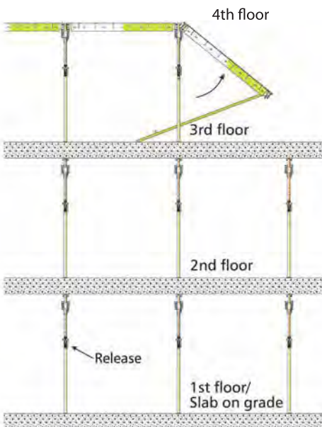
Step 7 Erect 4th floor with additional Props.
