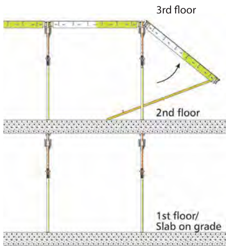
Step 4 Erect third floor with additional Props. Leave TABLA Backprops undisturbed.
